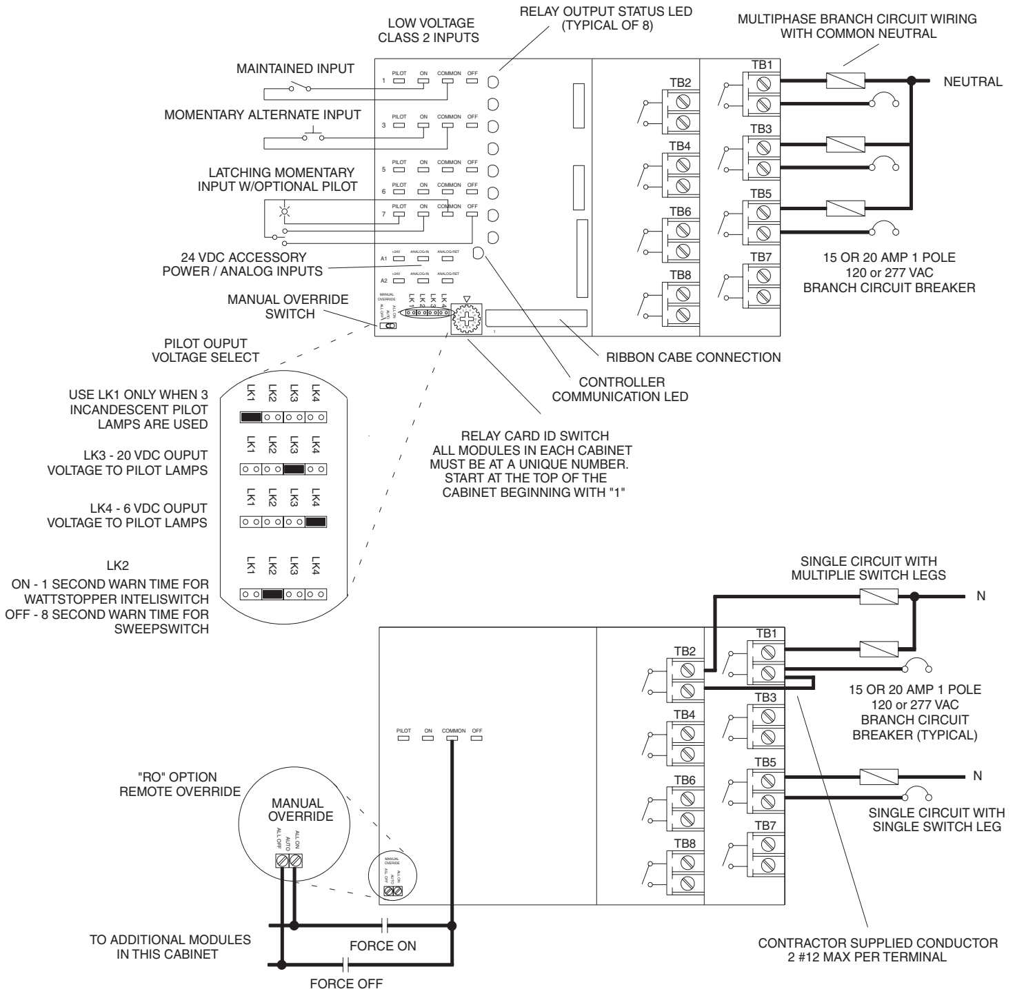
Figure 1 - SYPM 8R Wiring Detail
